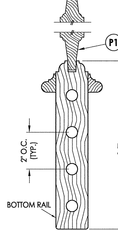
3 2 VERTICAL CROSS SECTION
